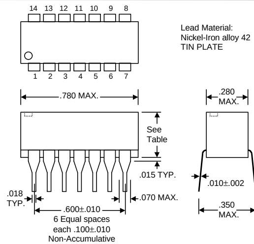
Package Dimensions
