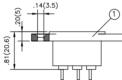
Countersunk Ear
