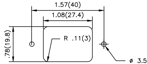
For Front Mounting Use Panel Cut-Out
