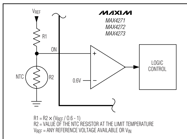
Figure 11. Temperature Monitoring and Protection
