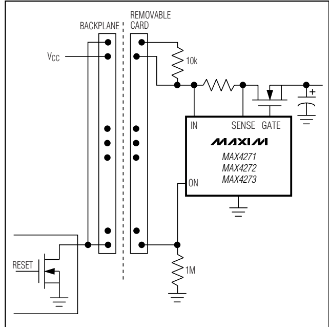
Figure 14. Fail-Safe Connector
