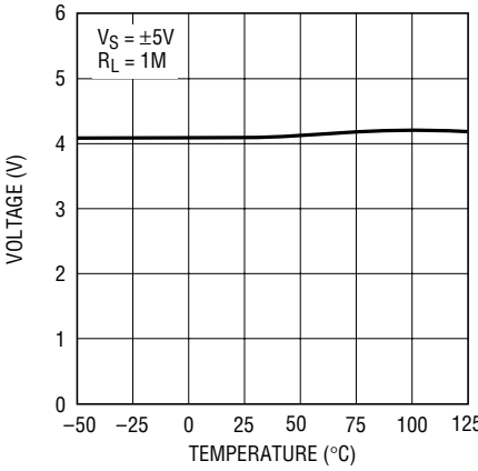
Positive Common Mode Limit vs Temperature
