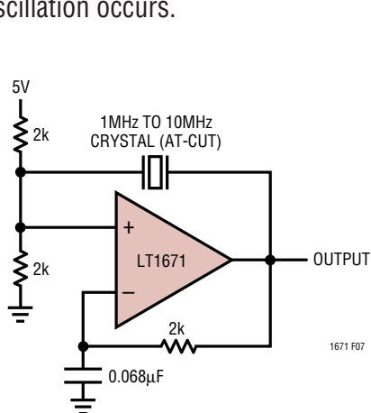
Figure 7. 1MHz to 10MHz Crystal Oscillator
