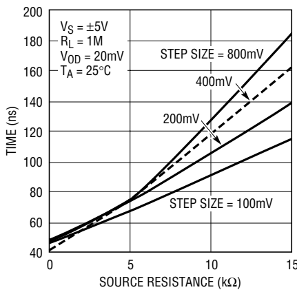
Propagation Delay vs Source Resistance
