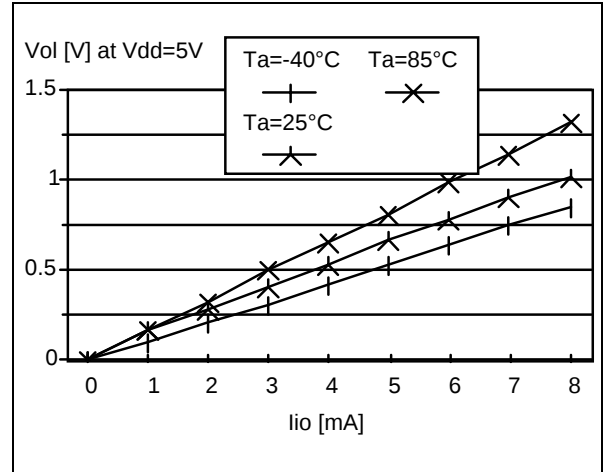
Figure 91. Typical V_{OL} at V_{DD}=5V ( \overline{\text{RESET}} )
