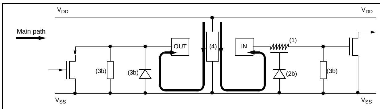
Figure 80. Multisupply Configuration
