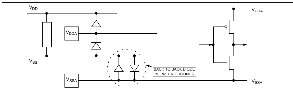
Figure 80. Multisupply Configuration
