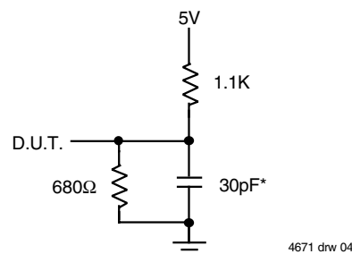
Figure 2. Output Load
