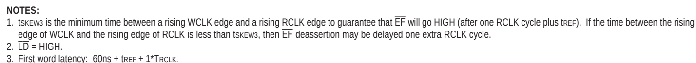
Figure 8. Read Cycle, Empty Flag and First Data Word Latency Timing (IDT Standard Mode)
