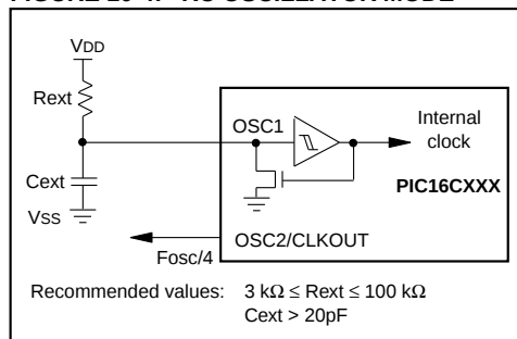
FIGURE 10-4: RC OSCILLATOR MODE
