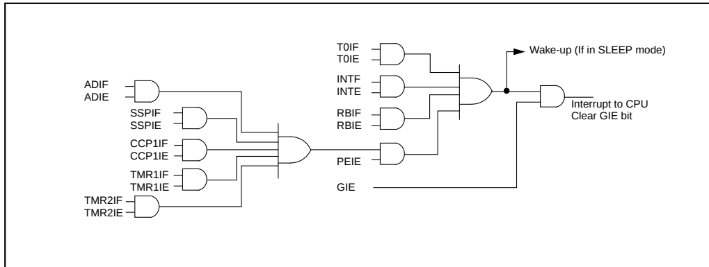
FIGURE 10-11: INTERRUPT LOGIC
