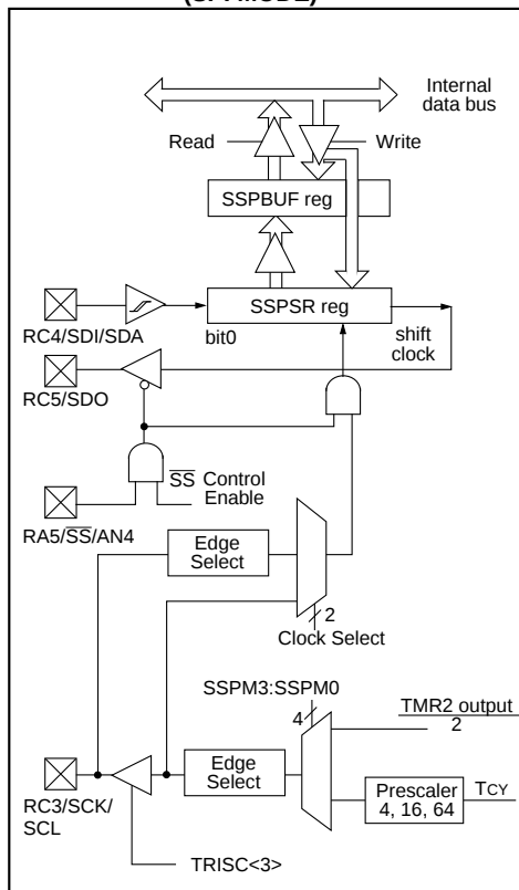
FIGURE 8-3: SSP BLOCK DIAGRAM (SPI MODE)
