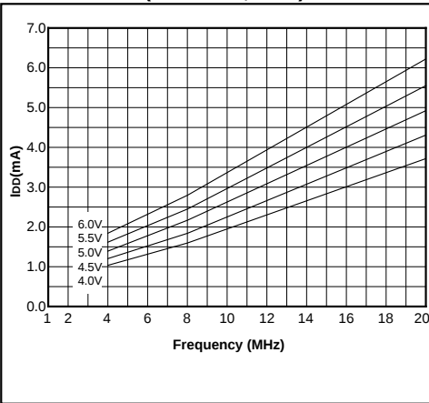
FIGURE 14-29: TYPICAL I_{DD} vs. FREQUENCY (HS MODE, 25°C)
