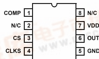
ISL6729 (8-PIN SOIC, MSOP) TOP VIEW
