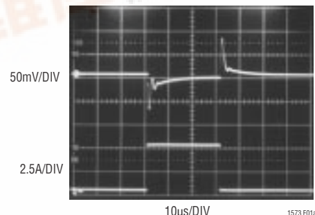
Transient Response for 0.2A to 5A Output Load Step
