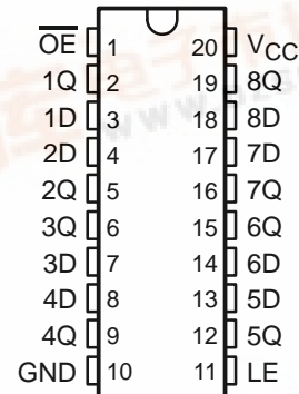
CD54HCT373 ... F PACKAGE CD74HCT373 ... E OR M PACKAGE (TOP VIEW)
