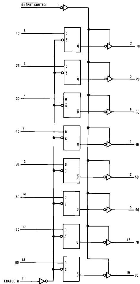
Logic Diagram
