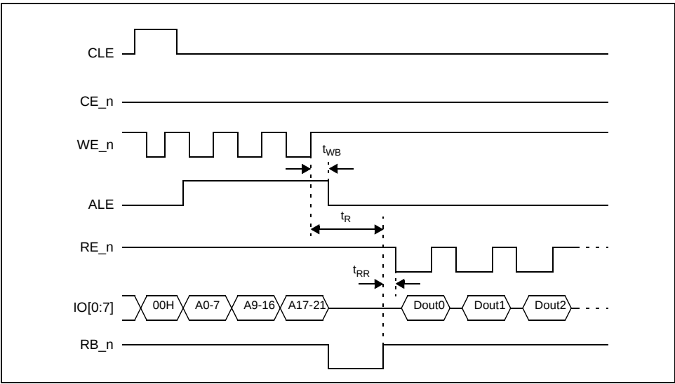
Figure 10: Read operation
