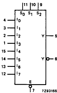
Fig.2 Logic symbol.
