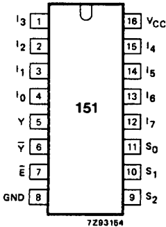
Fig.1 Pin configuration.
