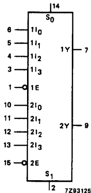
Fig.2 Logic symbol.
