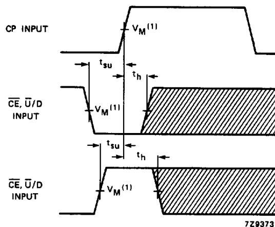
Fig.17 Waveforms showing the set-up and hold times from the count enable and up/down inputs ( \overline{\text{CE}} , \overline{\text{U/D}} ) to the clock (CP).
