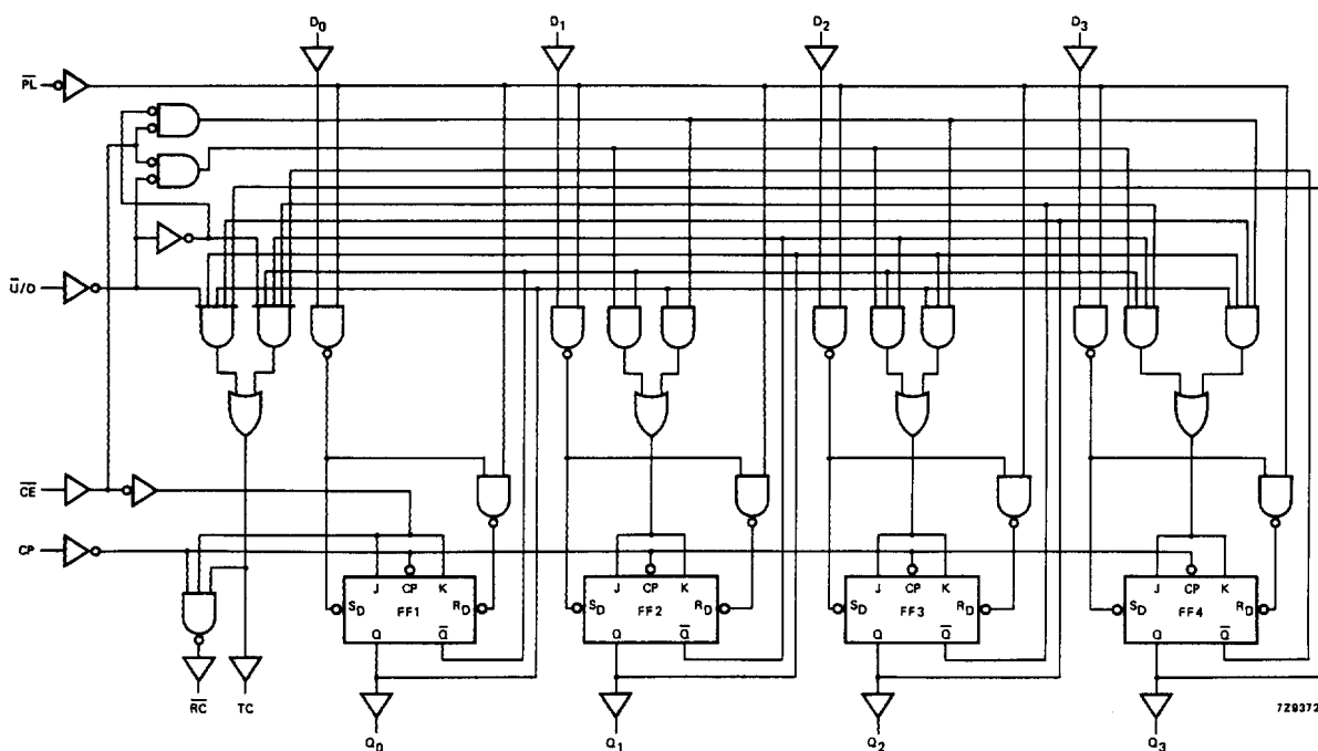
Fig.9 Logic diagram.
