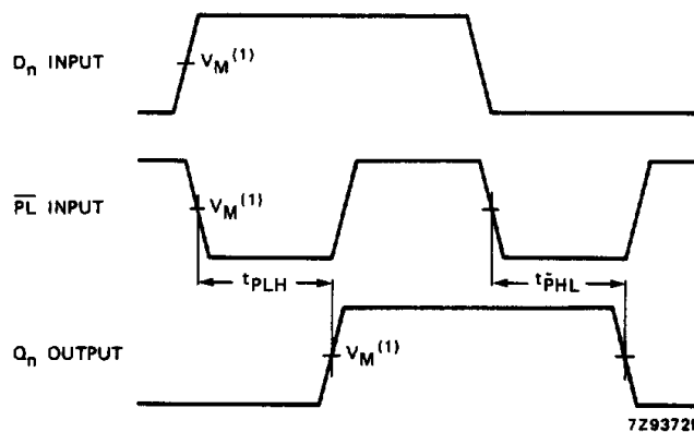
Fig.13 Waveforms showing the input ( \overline{\text{PL}} ) to output ( Q_n ) propagation delays.
