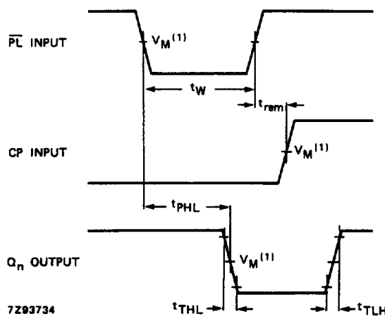
Fig.15 Waveforms showing the parallel load input ( \overline{\text{PL}} ) pulse width, removal time to clock ( \text{CP} ) and the output ( Q_n ) transition times.
