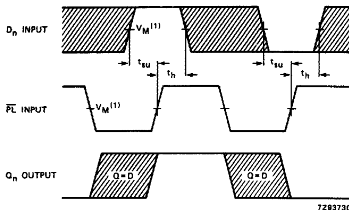
Fig.16 Waveforms showing the set-up and hold times from the parallel load input ( \overline{\text{PL}} ) to the data input ( D_n ).
