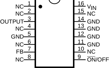
16-LEAD DIP (N)
