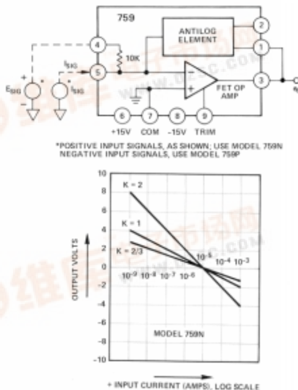
Figure1. Functional Block Diagram and Transfer Function
