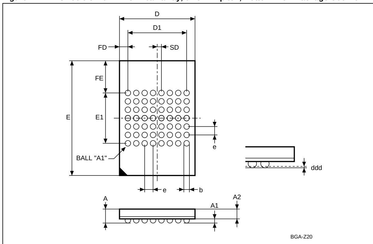
Figure 17. TFBGA56 6.5x10mm - 8x7 ball array, 0.75 mm pitch, Bottom View Package Outline
