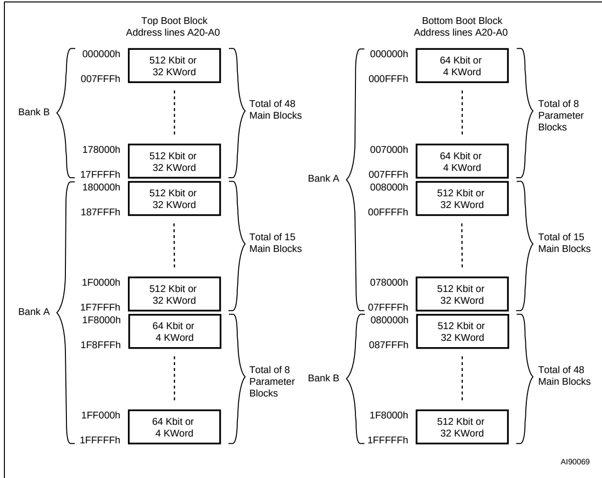
Figure 4. Memory Map
