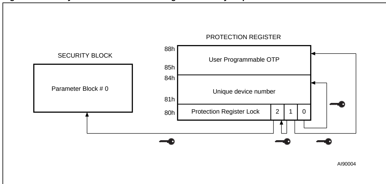
Figure 5. Security Block and Protection Register Memory Map
