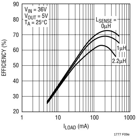
Figure 9. Efficiency and LT1777 Internal Dissipation for the Basic 5V Output Application
