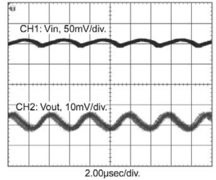
7812SR V_{IN} = 24\text{V} , I_{LOAD} = 40\text{mA}
