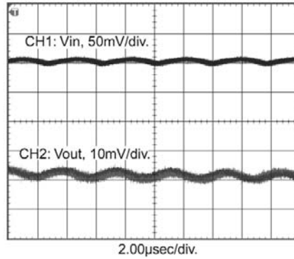
7805SR V_{IN} = 12\text{V} , I_{LOAD} = 50\text{mA}
