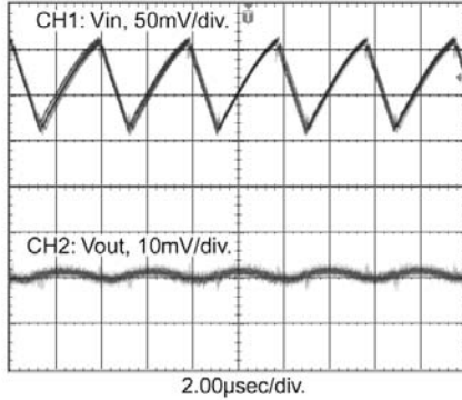
7803SR V_{IN} = 12\text{V} , I_{LOAD} = 500\text{mA}
