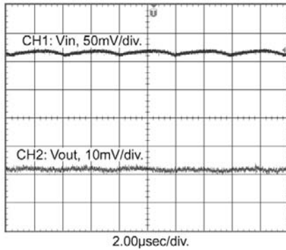
7803SR V_{IN} = 12\text{V} , I_{LOAD} = 50\text{mA}
