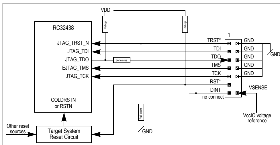
Figure 23 Target System Electrical EJTAG Connection
