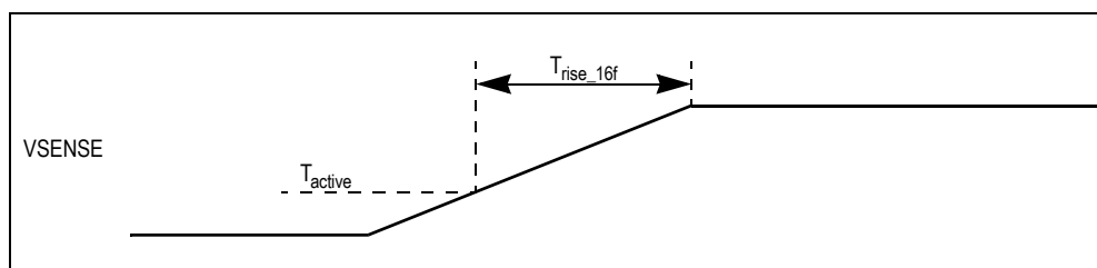
Figure 24 Voltage Sense Signal Timing
