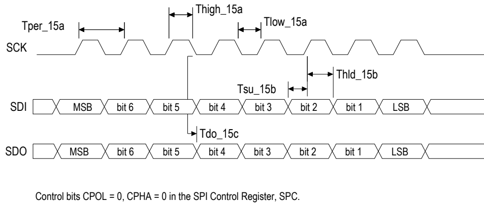
Figure 19 SPI AC Timing Waveform — Clock Polarity 0, Clock Phase 0
