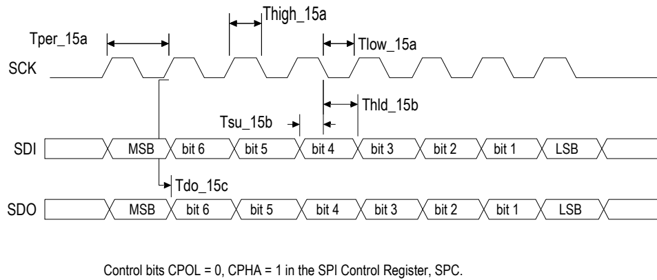
Figure 20 SPI AC Timing Waveform — Clock Polarity 0, Clock Phase 1
