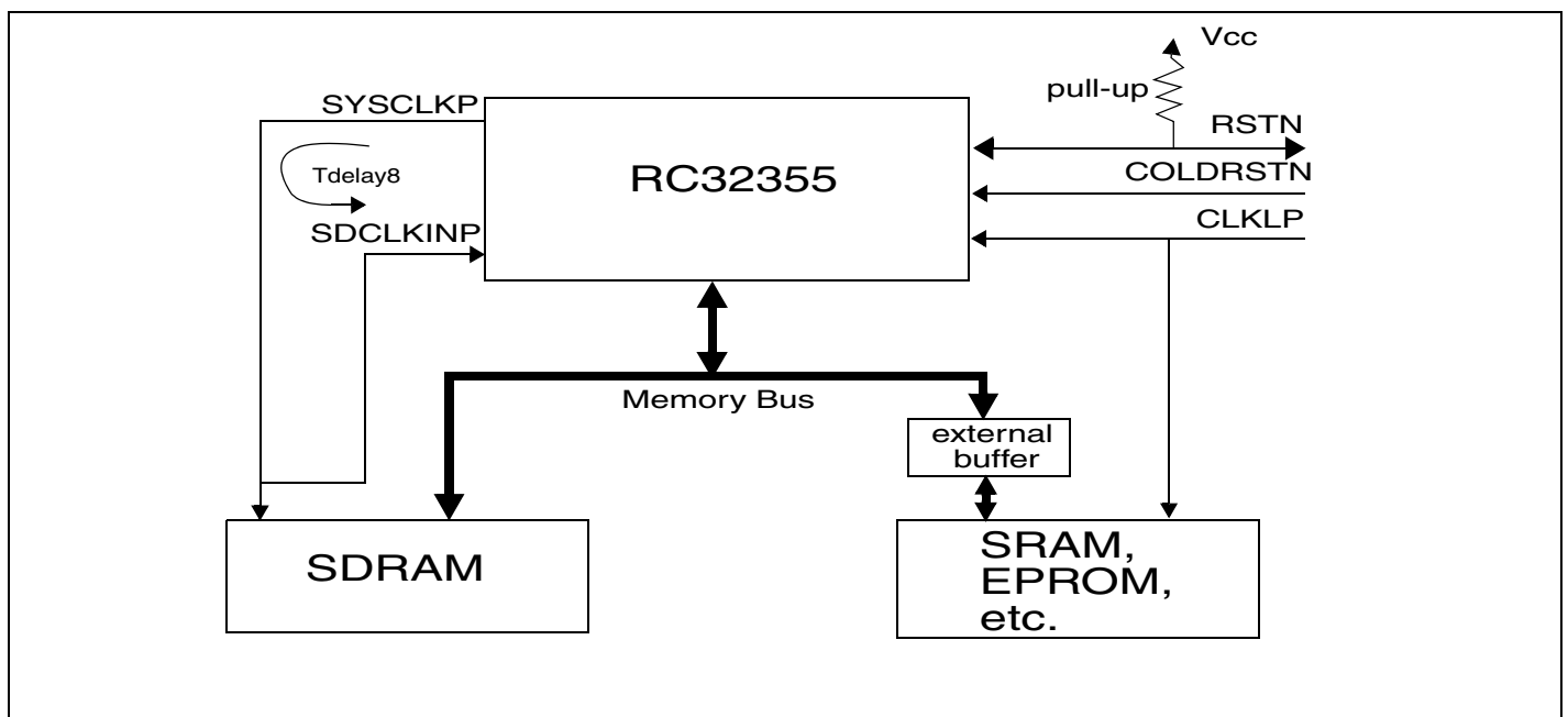
Figure 9 SYCLKP - SDCLKINP Relationship
