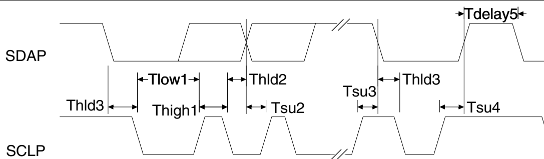
Figure 18 I²C AC Timing Waveform
