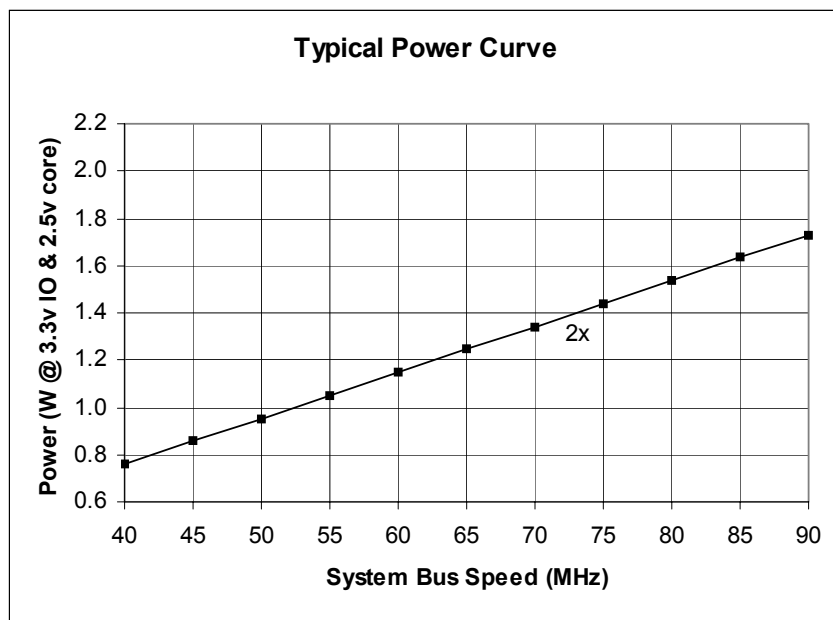
Figure 23 Typical Power Usage
