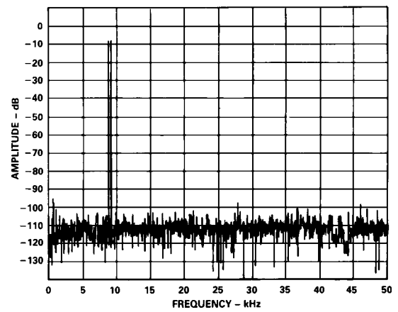
Figure 17. Nonaveraged IMD Plot for f_{\text{IN}} = 9.08 \text{ kHz} ( f_a ), 9.58 \text{ kHz} ( f_b ) at 128 kSPS
