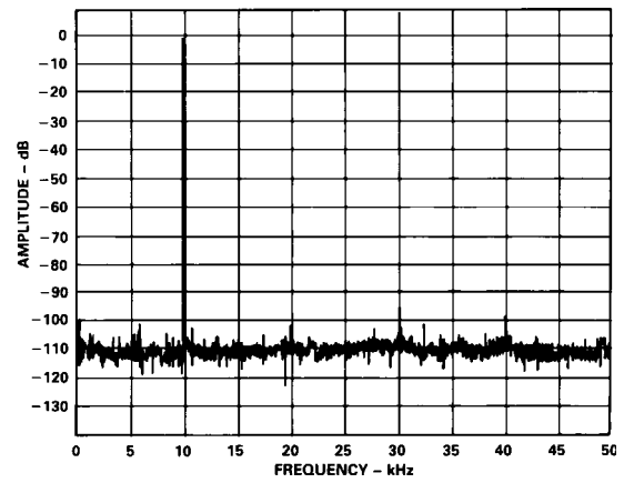
Figure 16. 5-Plot Averaged 2048 Point FFT at 128 kSPS, f_{\text{IN}} = 10.009 \text{ kHz}
