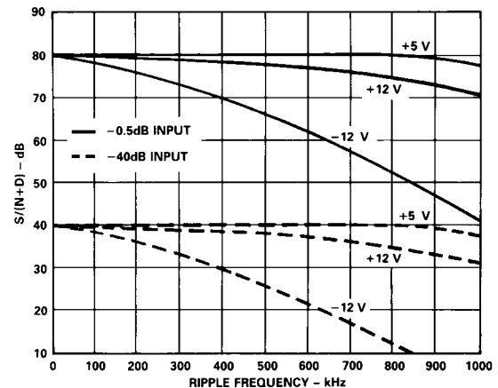
Figure 18. Power Supply Rejection ( f_{\text{IN}} = 10 \text{ kHz} , f_{\text{SAMPLE}} = 128 \text{ kSPS} , V_{\text{RIPPLE}} = 0.1 \text{ V p-p} )
