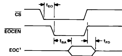
Figure 2. Output Timing
