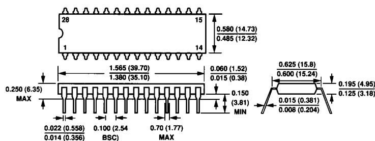
28-Lead Plastic DIP Package (N-28)
