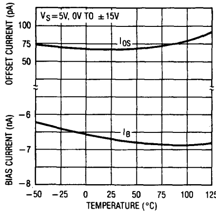
Input Bias and Offset Currents vs Temperature
