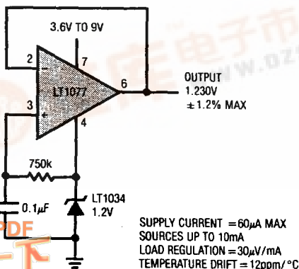
Self Buffered Micropower Reference
