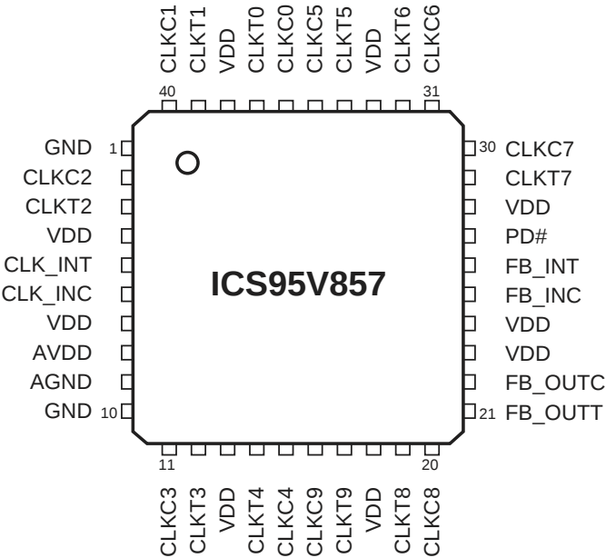
40-Pin MFL
