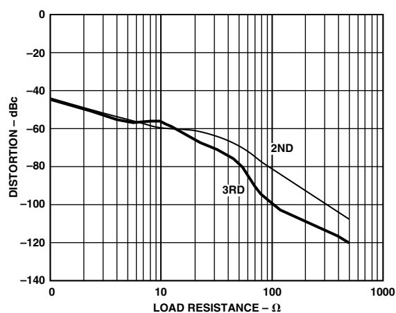
Figure 19. Distortion vs. R_L , V_S = \pm 2.5V , G = +2 , V_{OUT} = 2V_{p-p} , f = 1\text{ MHz}
