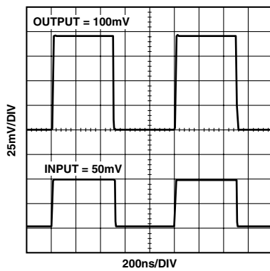
Figure 5. 100 mV Step Response; G = +2 , V_S = \pm 2.5 \text{ V} or \pm 6 \text{ V} , R_L = 100 \Omega
