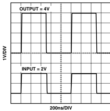
Figure 6. 4 V Step Response; G = +2 , V_S = \pm 6 \text{ V} , R_L = 100 \Omega
