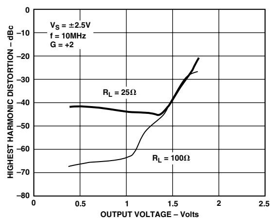
Figure 21. Distortion vs. Output Voltage, V_S = \pm 2.5V , G = +2 , f = 10\text{ MHz}
