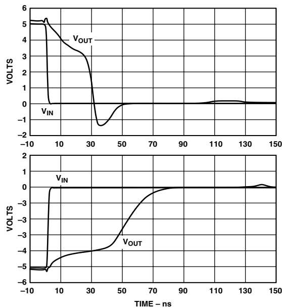
Figure 37. Overload Recovery; V_S = \pm 6 V , G = +2 , R_L = 100 \Omega , V_{IN} = 5 V_{p-p} , T = 1 \mu s
