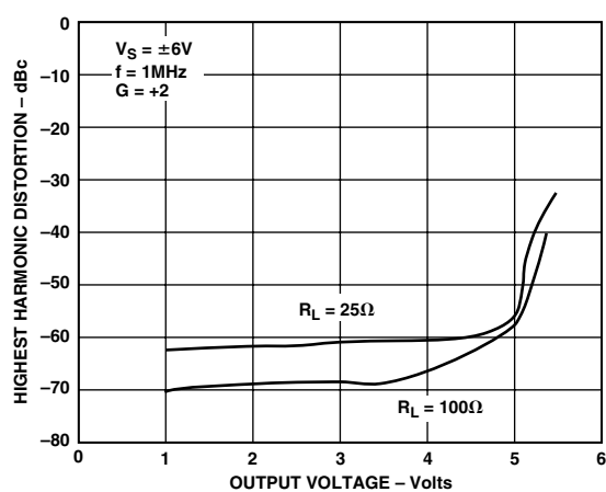
Figure 17. Distortion vs. Output Voltage, V_S = \pm 6V , G = +2 , f = 1\text{ MHz}
