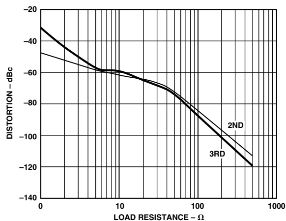
Figure 16. Distortion vs. R_L , V_S = \pm 6V , G = +2 , V_{OUT} = 2V_{p-p} , f = 1\text{ MHz}
