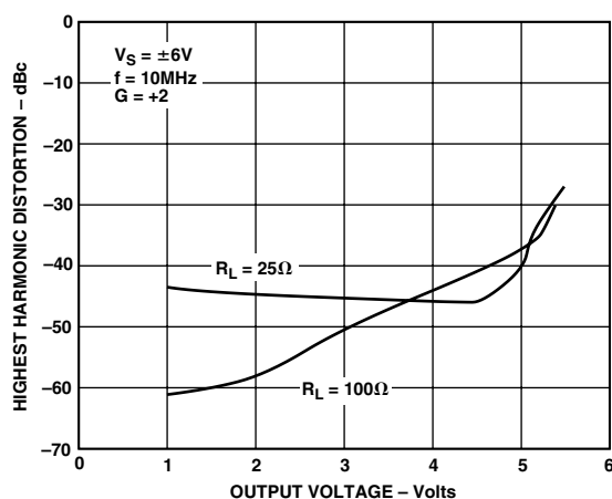
Figure 18. Distortion vs. Output Voltage, V_S = \pm 6V , G = +2 , f = 10\text{ MHz}
