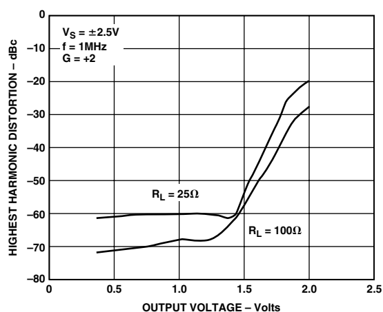
Figure 20. Distortion vs. Output Voltage, V_S = \pm 2.5V , G = +2 , f = 1\text{ MHz}
