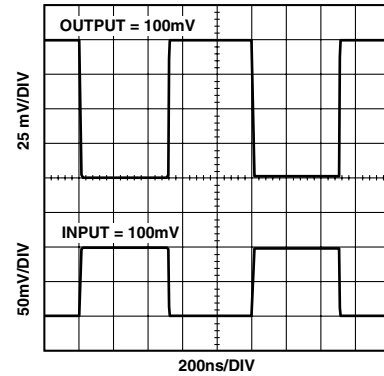
Figure 8. 100 mV Step Response; G = -1 , V_S = \pm 2.5 \text{ V} or \pm 6 \text{ V} , R_L = 100 \Omega
