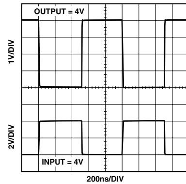
Figure 9. 4 V Step Response; G = -1 , V_S = \pm 6 \text{ V} , R_L = 100 \Omega
