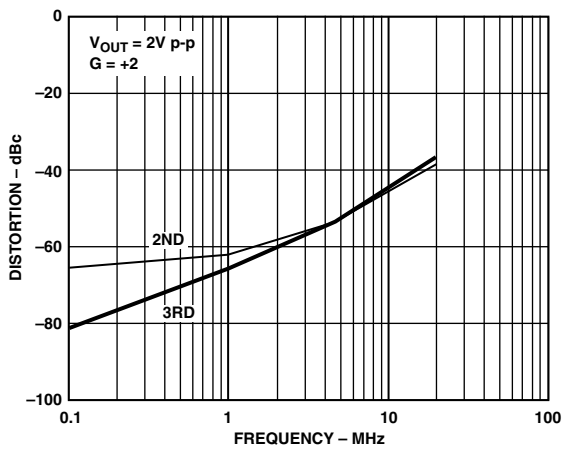
Figure 11. Distortion vs. Frequency; V_S = \pm 6V , R_L = 25\ \Omega
