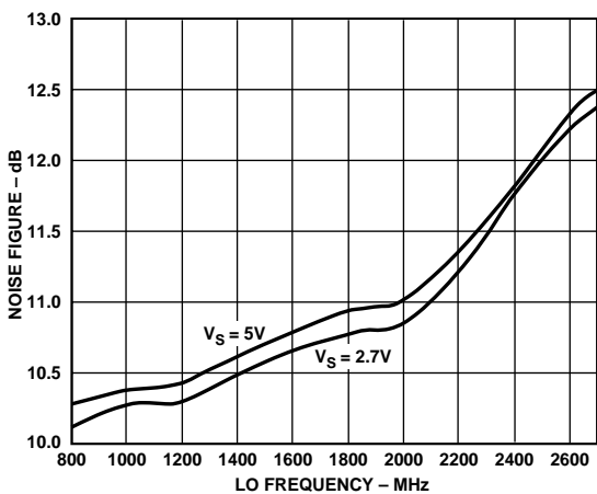
TPC 15. Noise Figure vs. LO Frequency ( F_{LO} ), Temperature = 25^\circ C , V_{GIN} = 0.2 V , F_{BB} = 1 MHz
