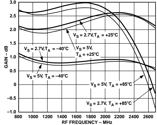
TPC 4. Gain vs. F_{LO} , V_{GIN} = 0.7 V, F_{BB} = 1 MHz
