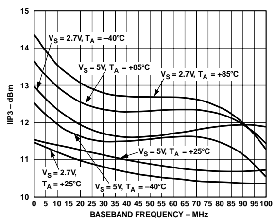
TPC 12. IIP3 vs. F_{BB} , V_{GIN} = 1.2\text{ V} , F_{LO} = 1900\text{ MHz}
