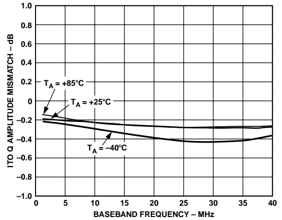
TPC 25. I/Q Amplitude Imbalance vs. F_{BB} , Temperature = 25°C, V_S = 5 V
