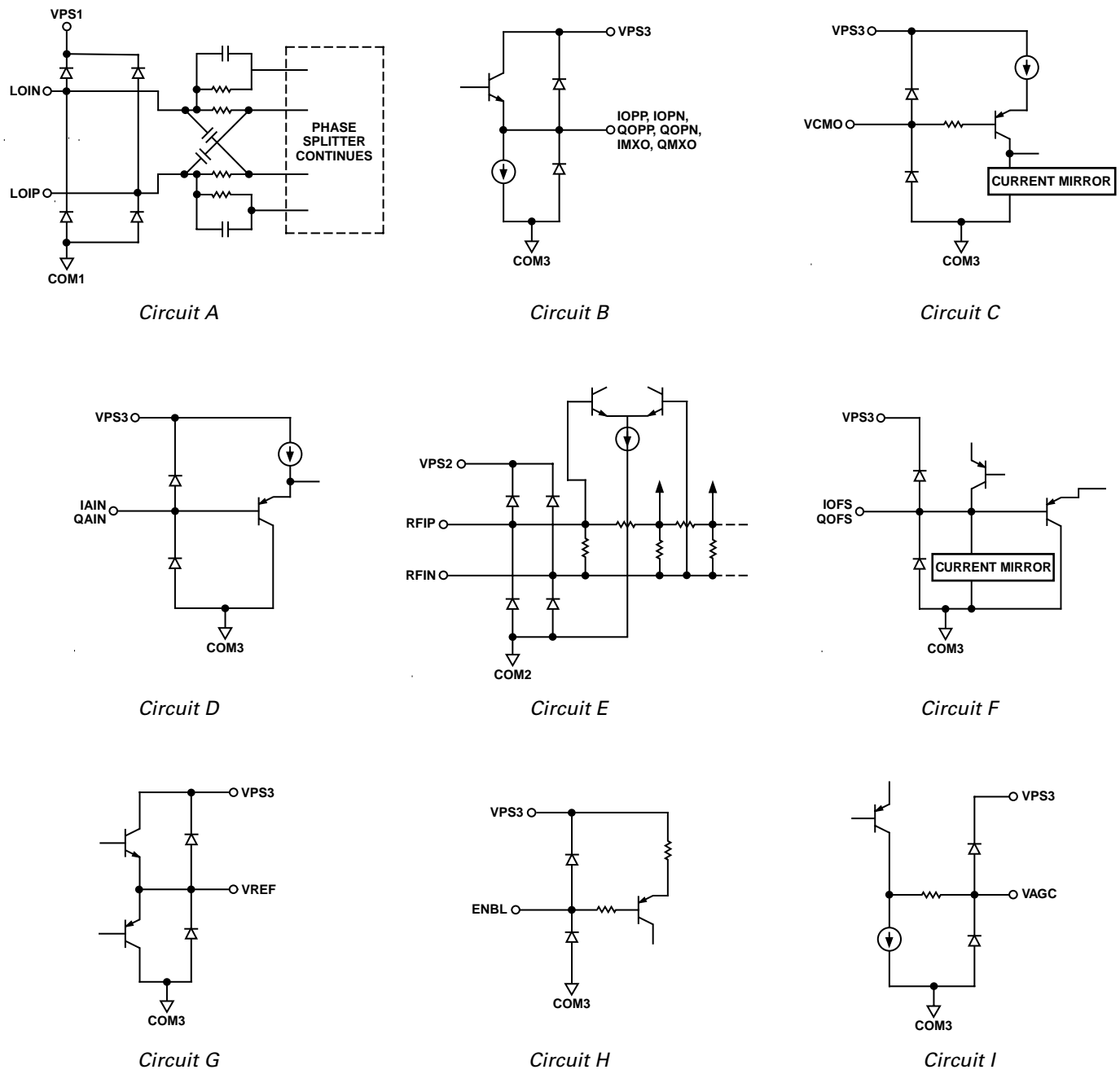
Figure 2. Equivalent Circuits
