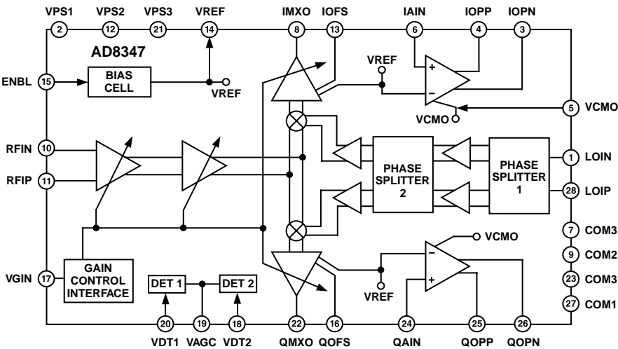
Figure 1. Block Diagram
