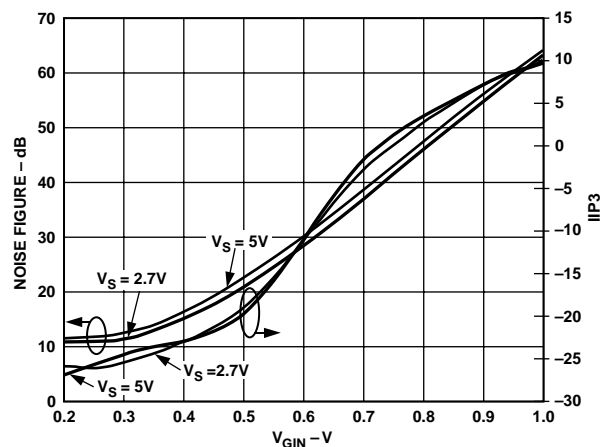
TPC 16. Noise Figure and IIP3 vs. V_{GIN} , Temperature = 25^\circ C , F_{LO} = 1900 MHz , F_{BB} = 1 MHz
