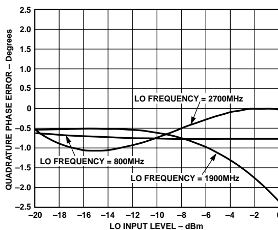
TPC 17a. Quadrature Error vs. LO Power Level, Temperature = 25^\circ C , V_{GIN} = 0.2 V , V_S = 5 V
