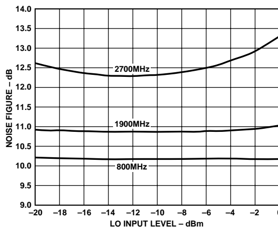
TPC 17b. Noise Figure vs. LO Input Level, Temperature = 25^\circ C , V_{GIN} = 0.2 V , V_S = 5 V
