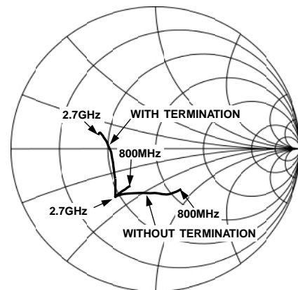
TPC 27. S_{11} of RFIN vs. F_{RF} , V_{GIN} = 0.7 V, V_S = 5 V
