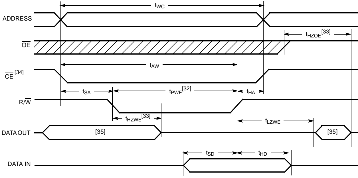
Write Cycle No. 2: CE Controlled Timing [29, 30, 31, 36]
