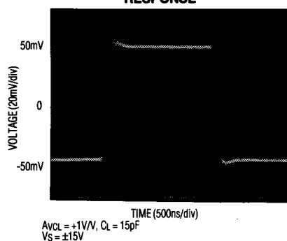
MAX437 SMALL-SIGNAL TRANSIENT RESPONSE
