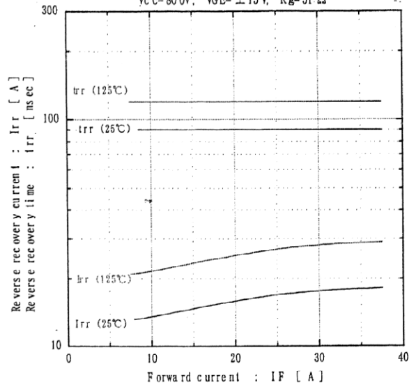
[ Inverter ] Reverse recovery characteristics (typ.) Vcc = 80.0V, VGE = ±15V, RG = 51Ω
