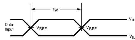
FIGURE 2. Voltage Waveforms - Pulse Duration
