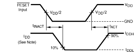
FIGURE 3. Voltage and Current Waveforms Inputs Active and Inactive Times
