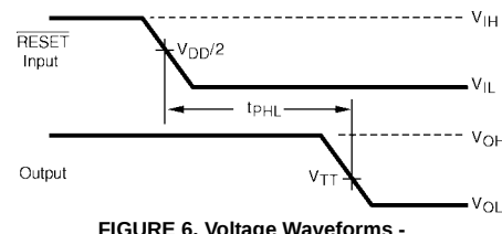
FIGURE 6. Voltage Waveforms - RESET Propagation Delay Times
