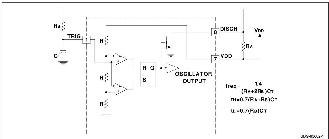
Figure 1. Oscillator Block Diagram
