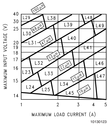
FIGURE 5. LM2677-12
