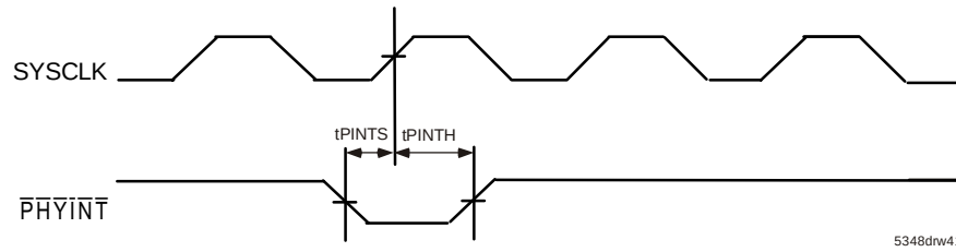
Figure 37 System Clock to PHYINT Propagation Delay
