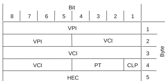
NNI Cell Header (five byte field)
