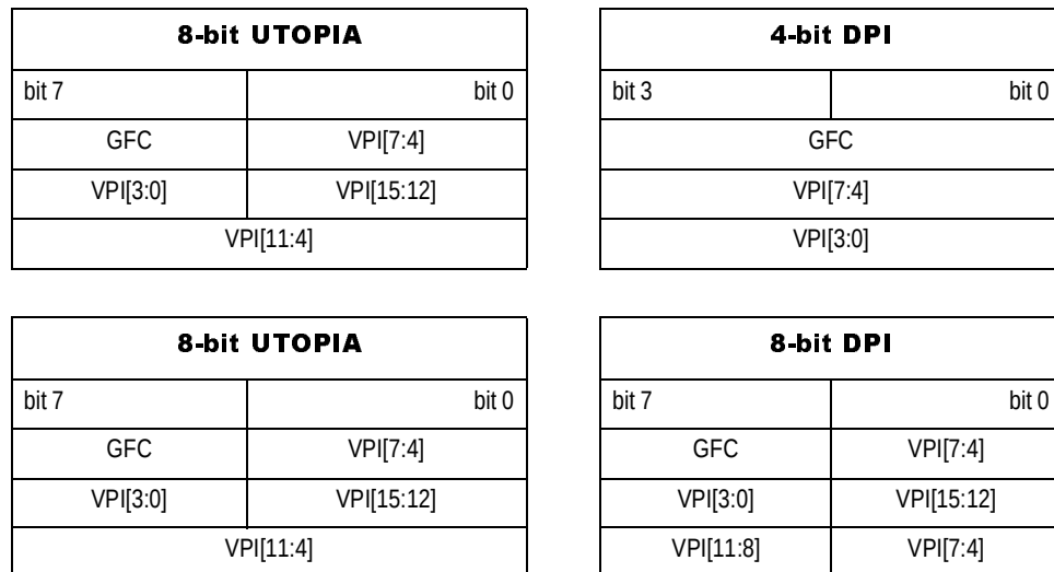
Figure 11 UTOPIA to DPI Conversion
