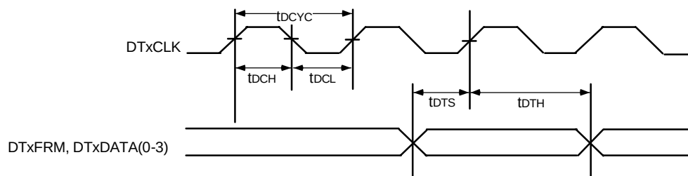
Figure 34 DPI Transmit Timing Waveform
