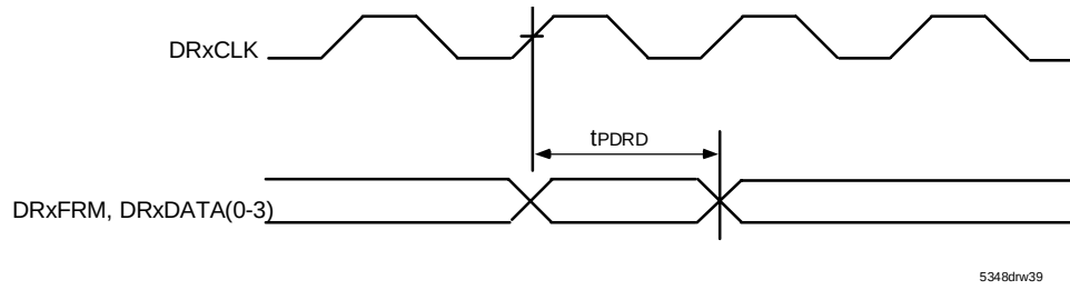
Figure 35 DPI Receive Timing Waveform
