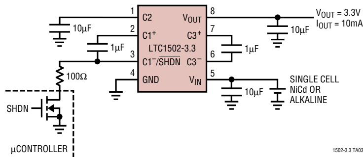
Single Cell to 3.3V DC/DC Converter with Shutdown
