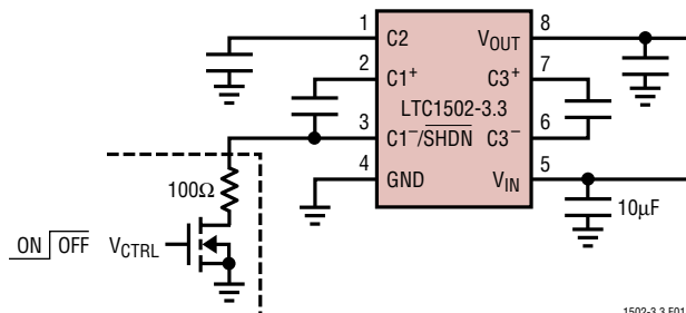
Figure 1. Pull-Down Circuitry for Shutdown
