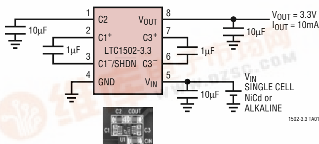
Single Cell to 3.3V DC/DC Converter
