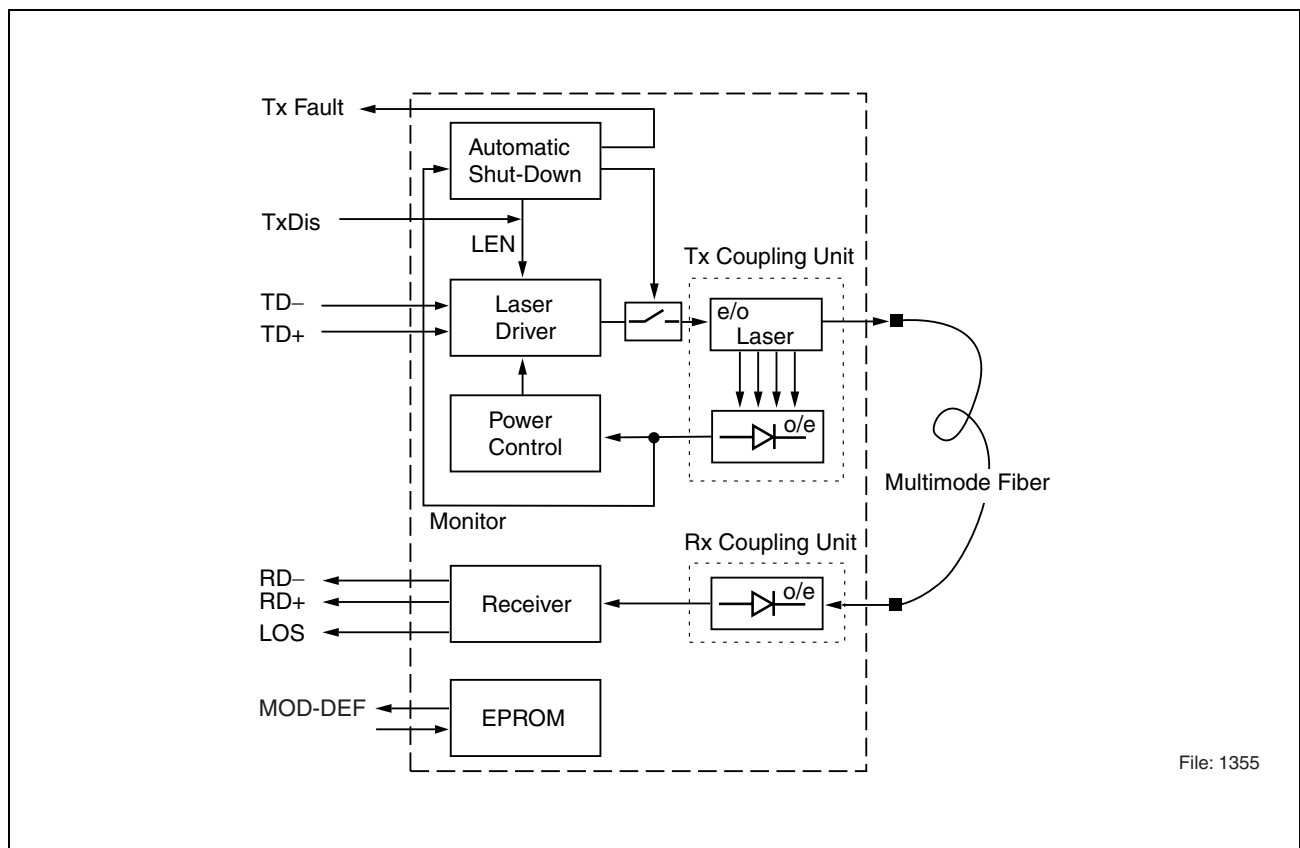
Figure 2 Functional Diagram
