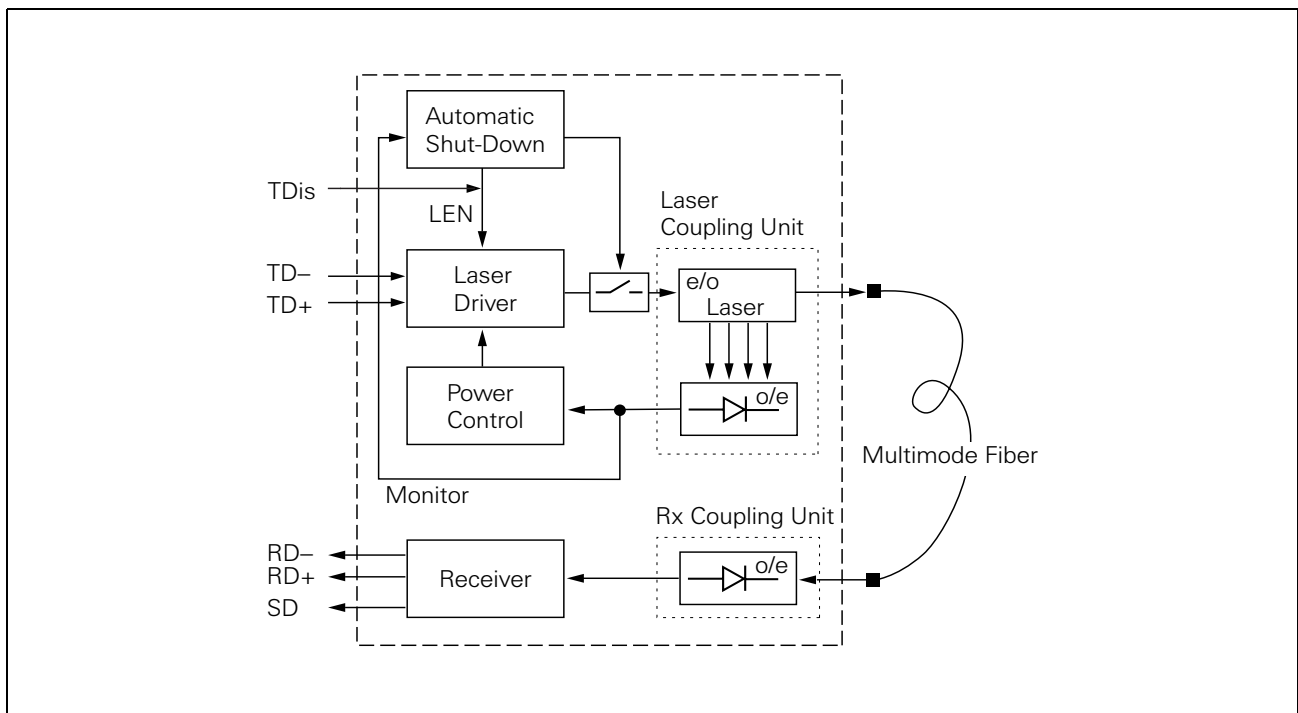
Figure 2 Functional Diagram
