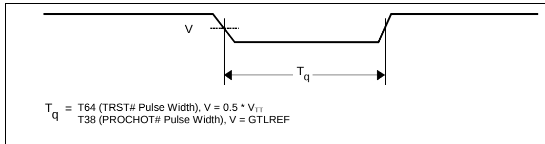
Figure 2-14. Test Reset (TRST#), Async GTL+ Input, and PROCHOT# Timing Waveform
