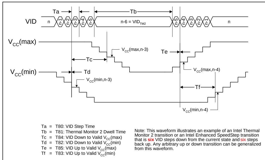
Figure 2-22. VID Step Times and V_{CC} Waveforms
