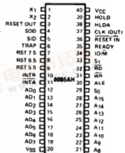
Figure 2. 8085AH Pin Configuration
