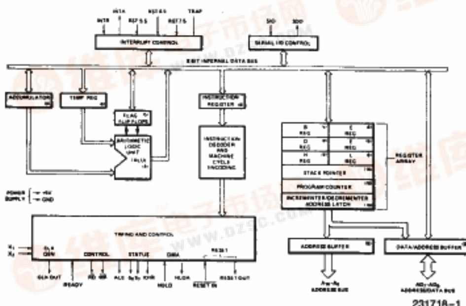
Figure 1. 8085AH CPU Functional Block Diagram
