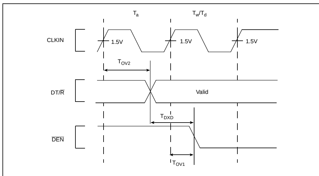
Figure 27. DT/\overline{R} and \overline{DEN} Timings Waveform
