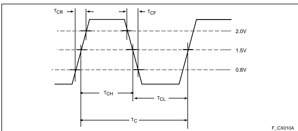
Figure 9. CLKIN Waveform
