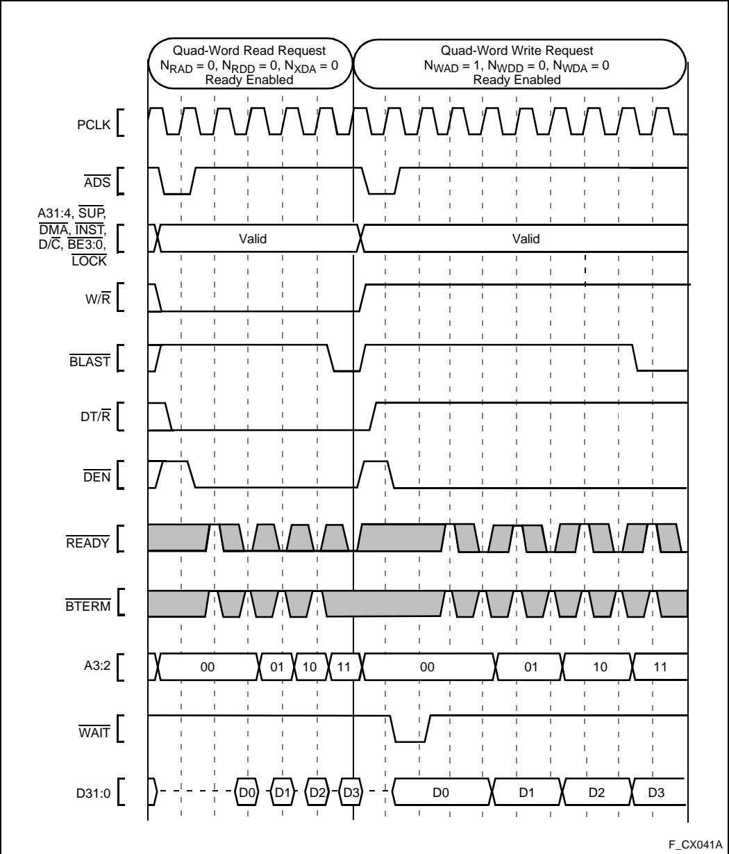
Figure 39. Using External \overline{\text{READY}}
