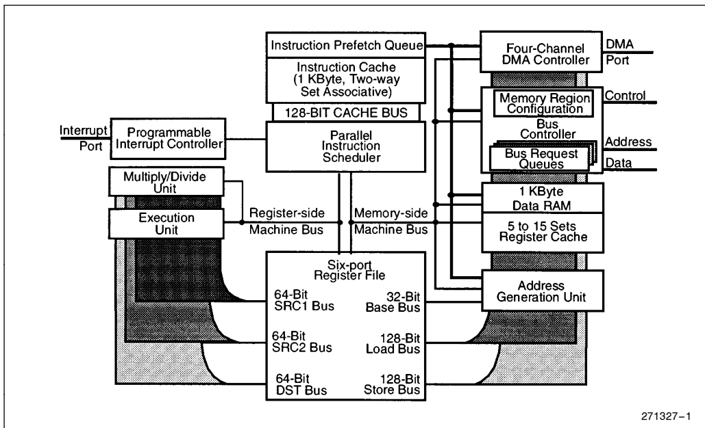
Figure 1. 80960CA Block Diagram
