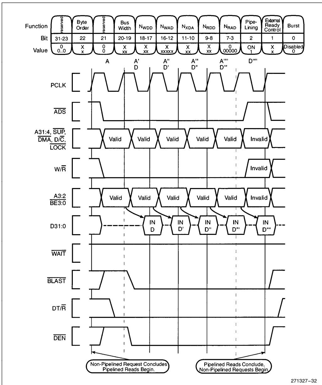
Figure 32. Non-Burst, Pipelined Read Request Without Wait States, 32-Bit Bus
