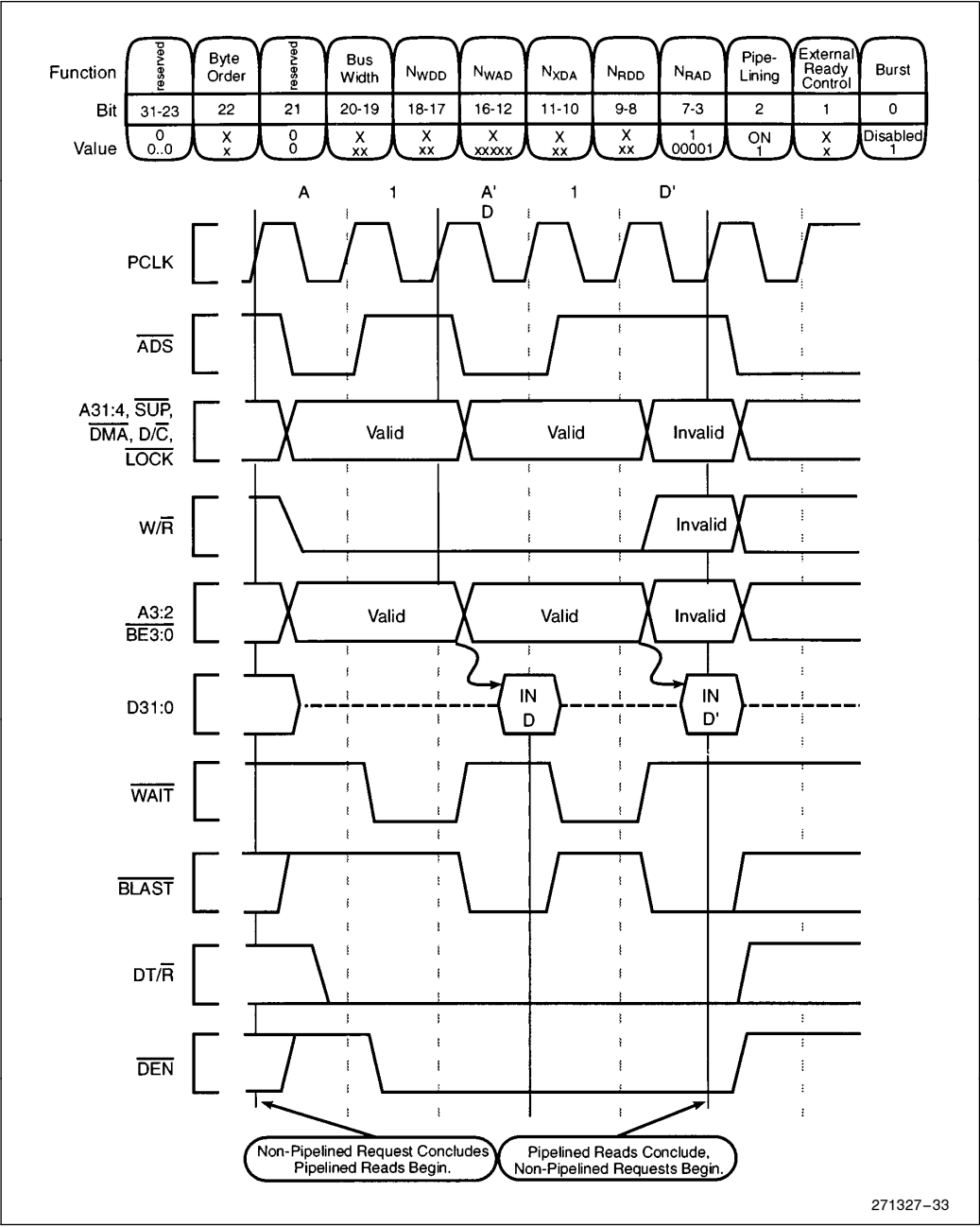
Figure 33. Non-Burst, Pipelined Read Request With Wait States, 32-Bit Bus
