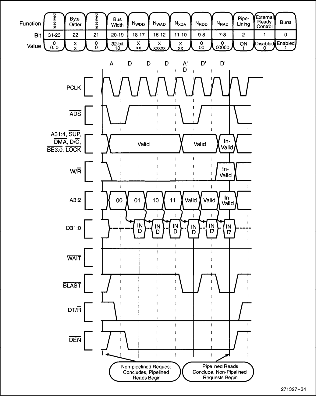
Figure 34. Burst, Pipelined Read Request Without Wait States, 32-Bit Bus
