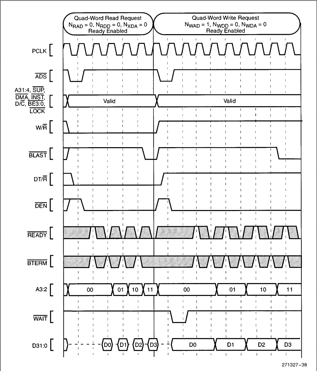
Figure 38. Using External \overline{\text{READY}}
