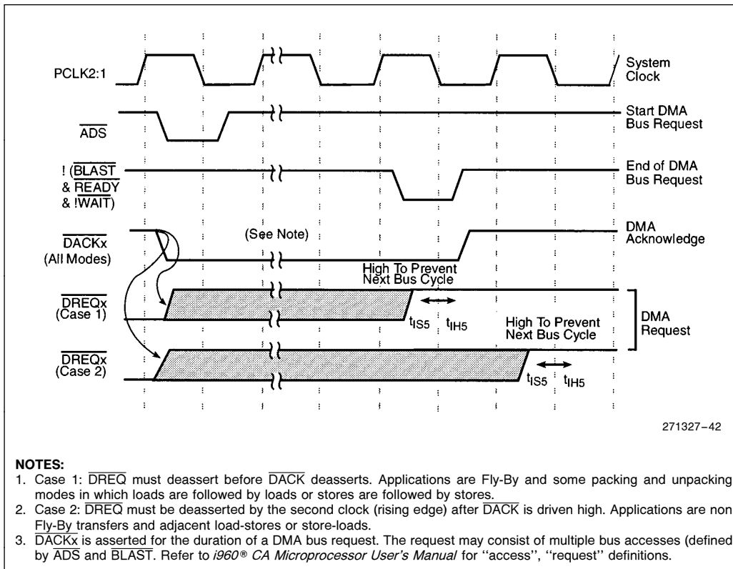
Figure 42. DREQ and DACK Functional Timing
