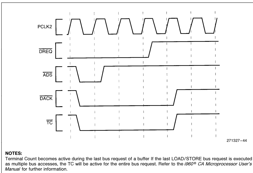
Figure 44. Terminal Count Functional Timing
