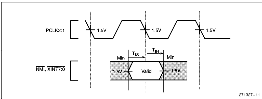
Figure 11. NMI, XINT7:0 Input Setup and Hold Waveform
