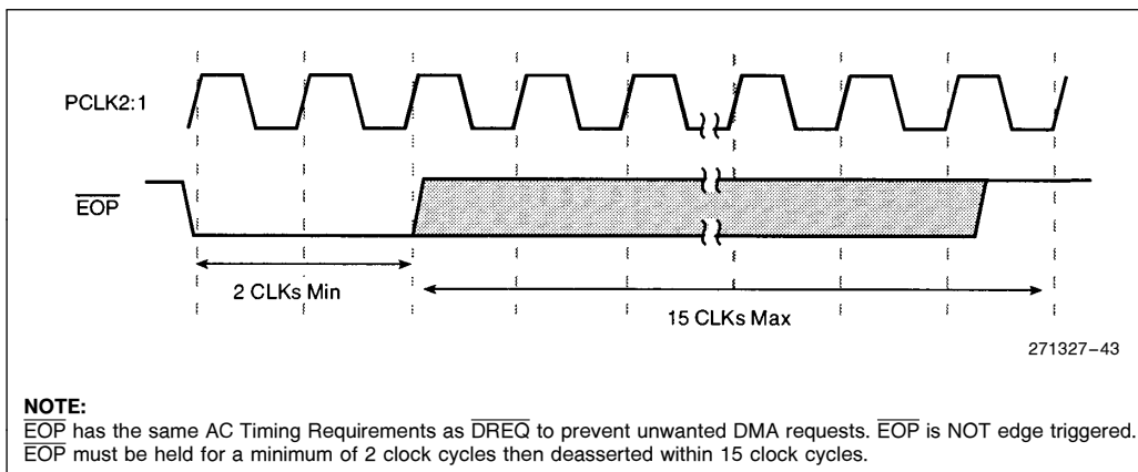
Figure 43. EOP Functional Timing
