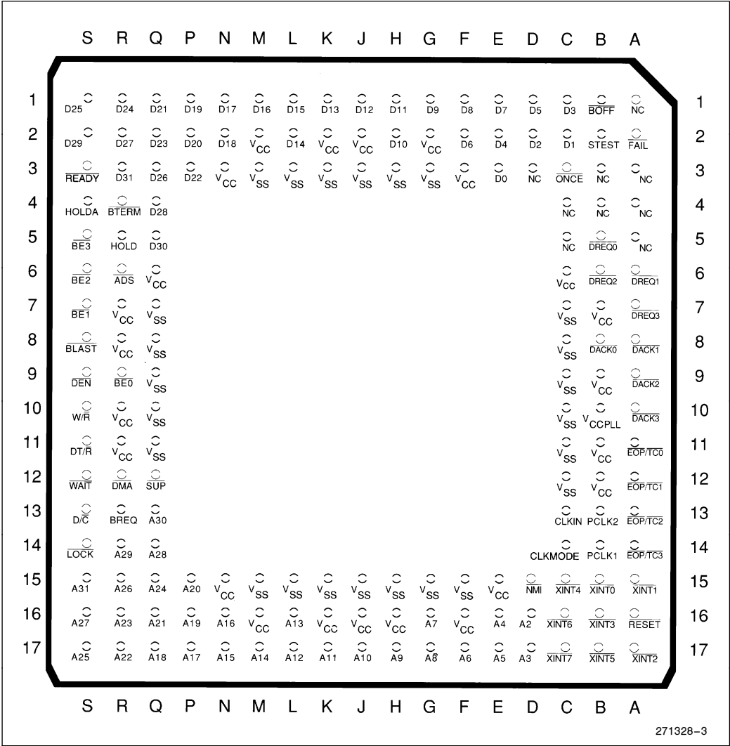
Figure 4a. 80960CF PGA Pinout (View from Top Side)
