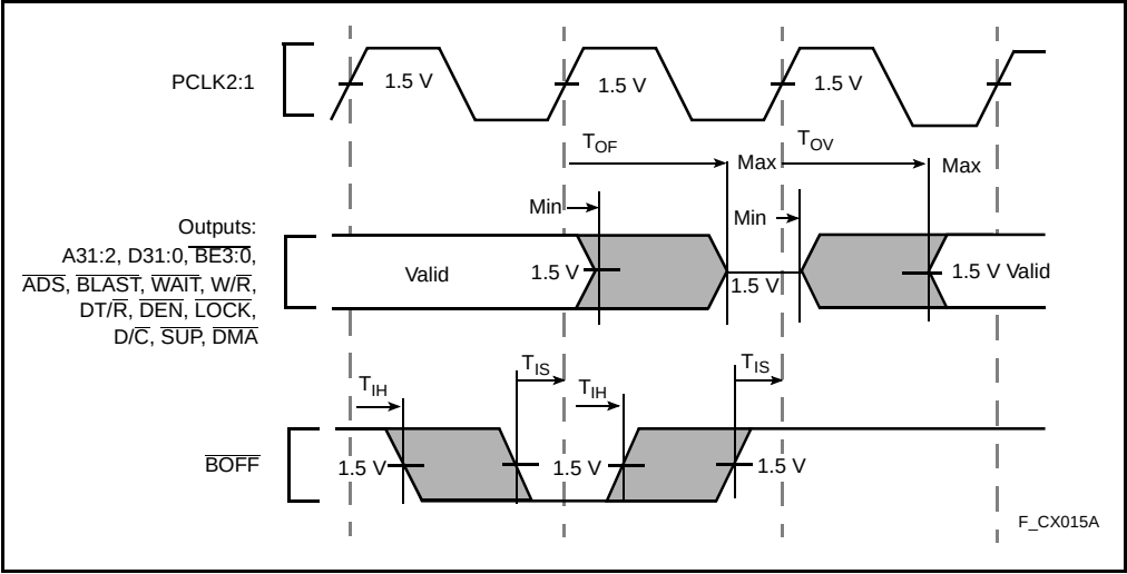
Figure 14. Bus Backoff (BOFF) Timings
