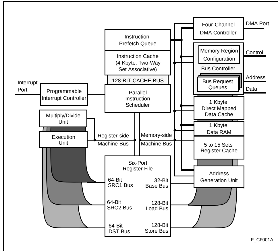
Figure 1. 80960CF Block Diagram
