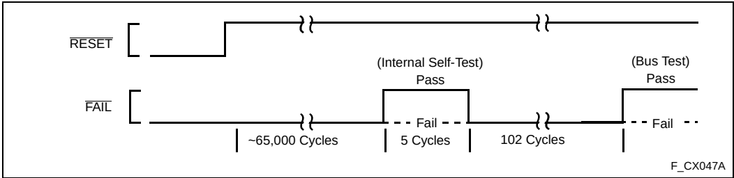
Figure 47. \overline{\text{FAIL}} Functional Timing
