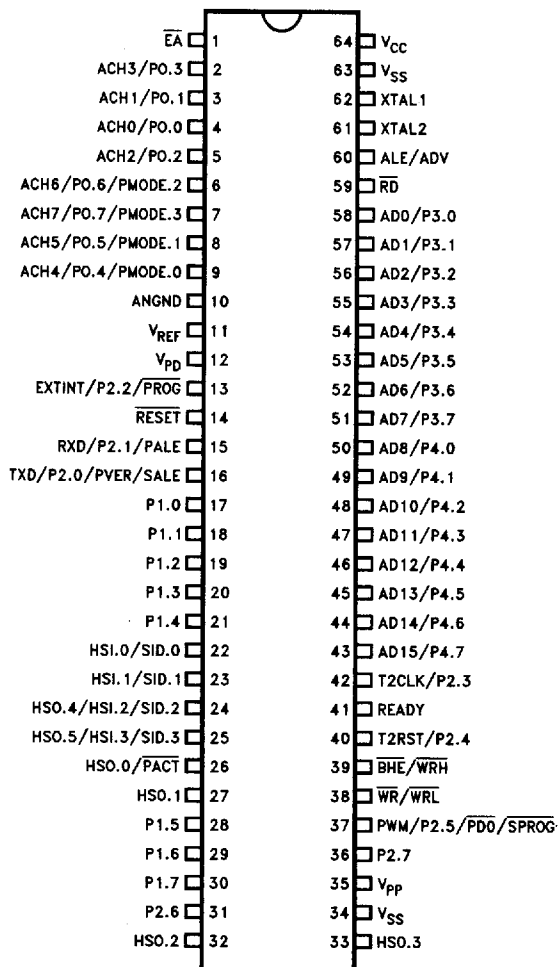
Figure 6. Shrink-DIP Package
