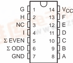
D OR N PACKAGE (TOP VIEW)
