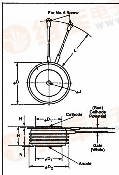
T82 Outline Drawing
