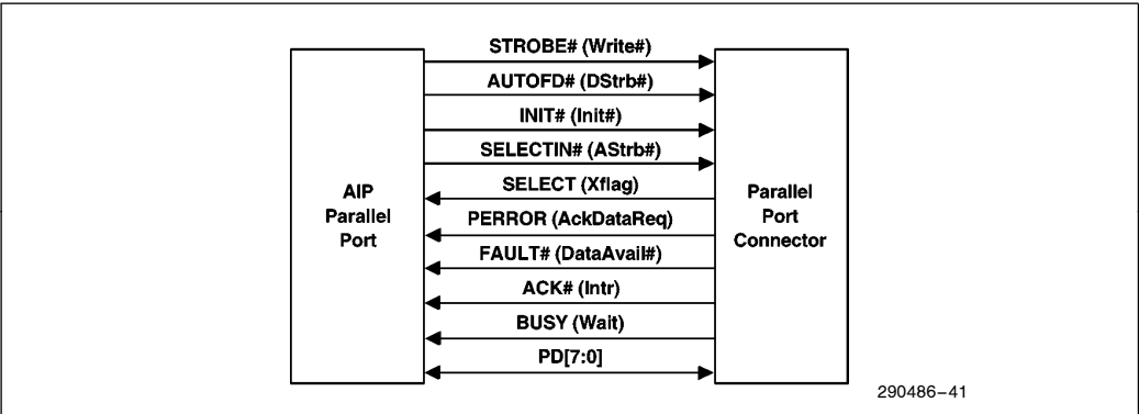
Figure 41. EPP Mode
