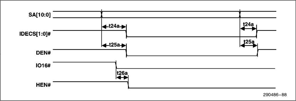
Figure 88. IDE Timing
