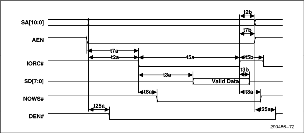
Figure 72. Host Read
