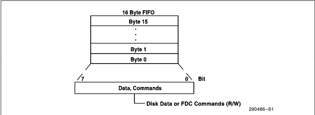
Figure 61. FDC FIFO
