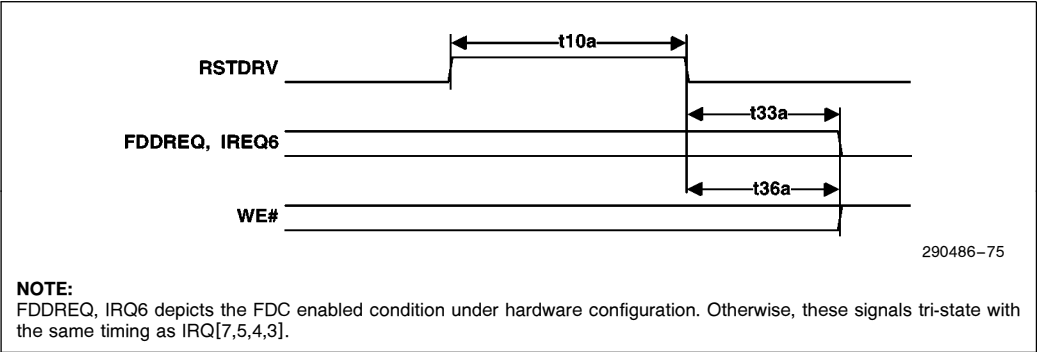
Figure 75. Reset Timing
