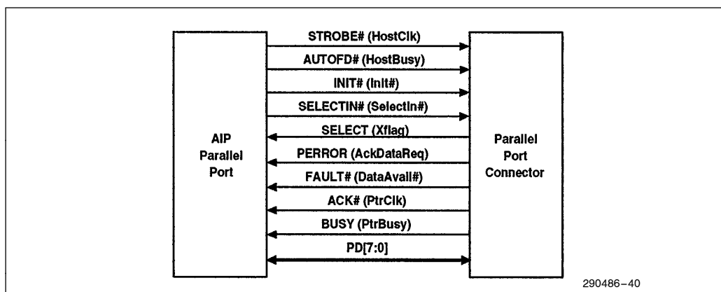
Figure 40. PS/2-Compatible Mode
