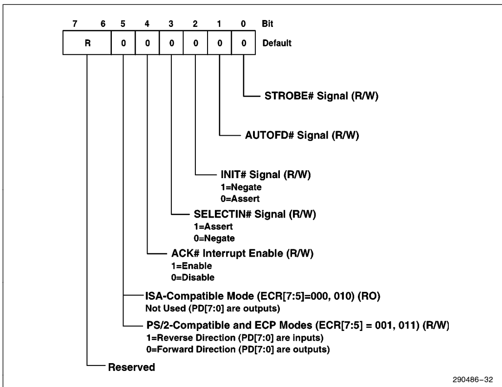
Figure 32. Control Register (ECP Mode)
