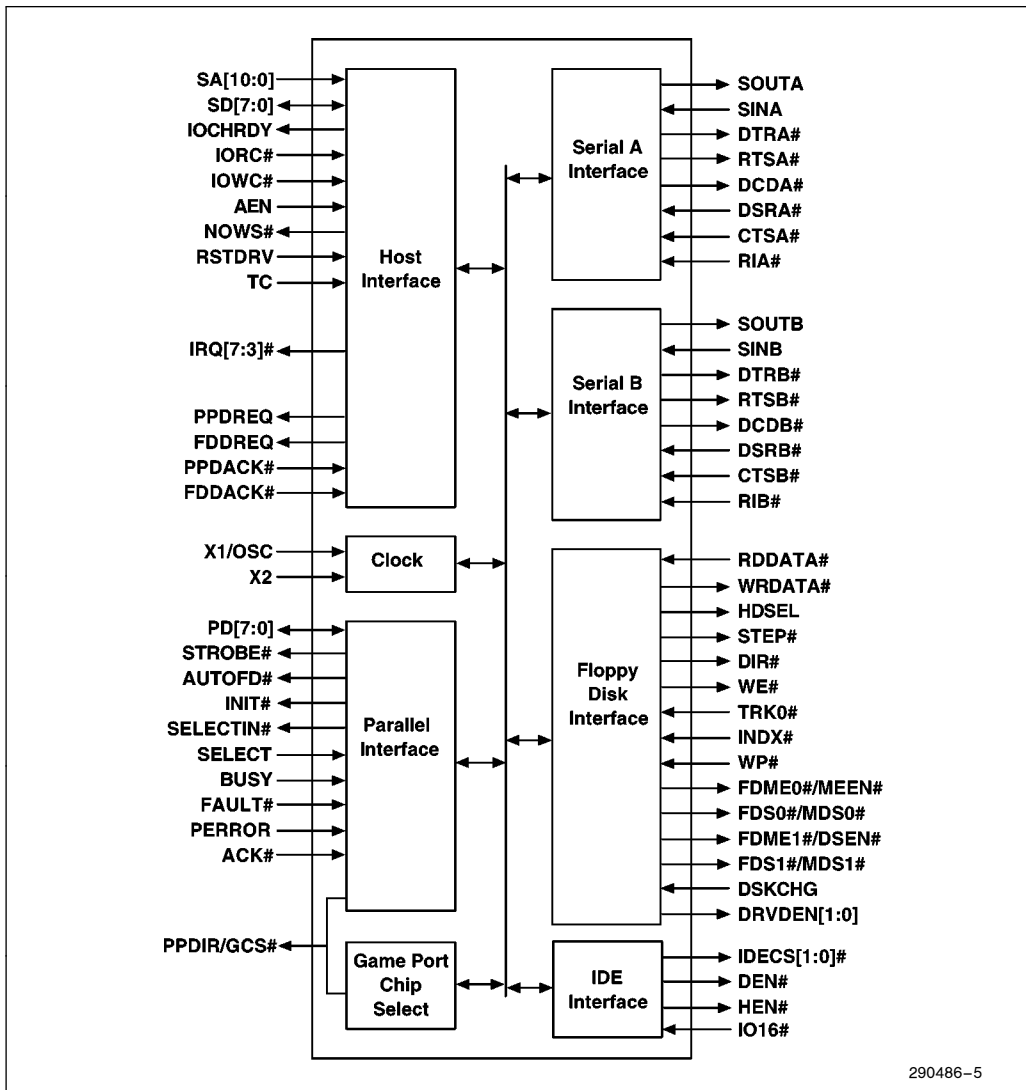
Figure 5. 82091AA Signals
