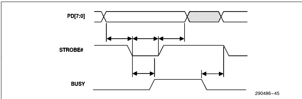
Figure 45. ISA-Compatible Timing
