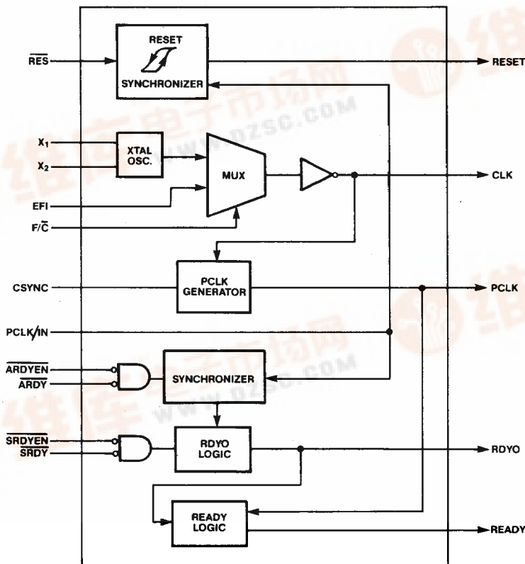
Figure 1. 82285 Block Diagram
