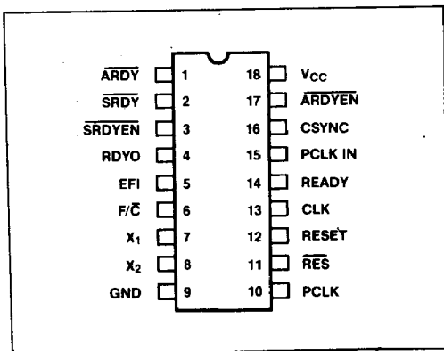
Figure 2. 82285 Pin Configuration
