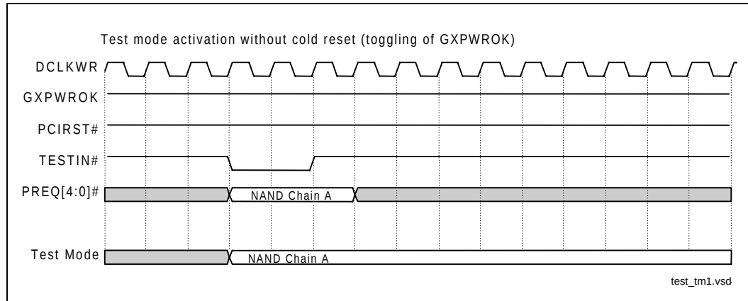
Figure 6-1. Waveform of Test Mode
