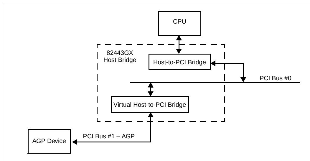
Figure 3-1. 82443GX PCI Bus Hierarchy
